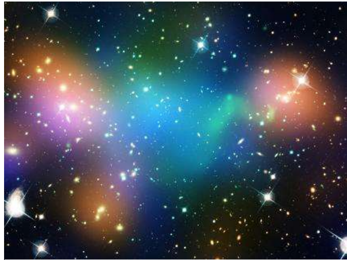
"Merging Galaxy Cluster Abell 520" Source: nasa.gov
